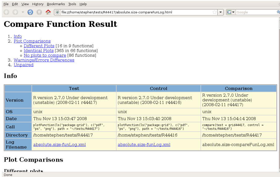
Figure 5.1: Information section of the grid comparison report.
