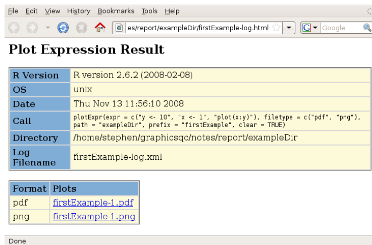
Figure 4.1: Report on a qcPlotExprResult object.
